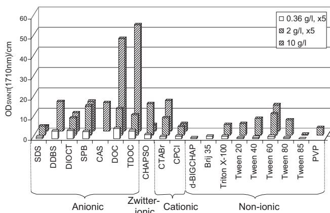
Figure 2. Peak SWNT absorbances (first van Hove transition at ~1710 nm) as a measure of relative SWNT concentration, for each surfactant and for different initial concentrations of the raw material, after settling for 3 days. Data for the lower two concentrations are magnified 5 times for clarity. For these two data series, the SWNT material was obtained from a common ethanol stock dispersion, while for the higher concentration data the as-produced raw material was used directly (see Sec. 4.1.).
