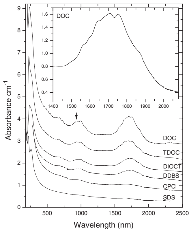
Figure 3. Absorption spectra of SWNT dispersions with different surfactants (starting from 10 mg raw material in 1 mL D 2 O) after ultracentrifugation. No background subtraction (other than the baseline correction for solvent and surfactant absorption) was applied. Spectra are shifted vertically (steps of 0.5, starting from zero for SDS) for clarity. An arrow marks the excitation wavelength (930 nm) used for the fluorescence measurements of Figure 4.
