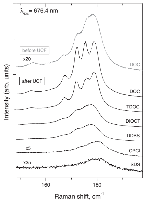
Figure 5. Radial breathing mode region of the Raman spectra, excited at 676.4 nm, for the same SWNT dispersions as in Figure 3, as well as for the SWNT/DOC solution before UCF. Spectra for CTABr and Tween 60 (not shown) were almost identical in shape to that for CPCI, but with higher intensities. The instrumental resolution was 0.34 cm -1 .
