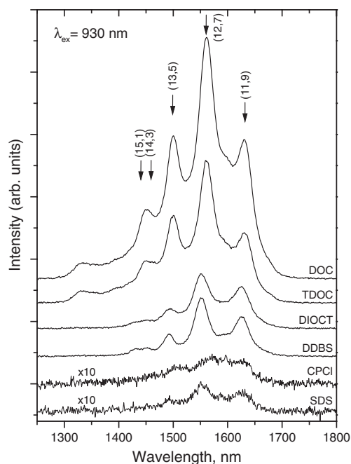
Figure 4. Fluorescence spectra, excited at 930 nm, of the same SWNT dispersions as in Figure 5.
