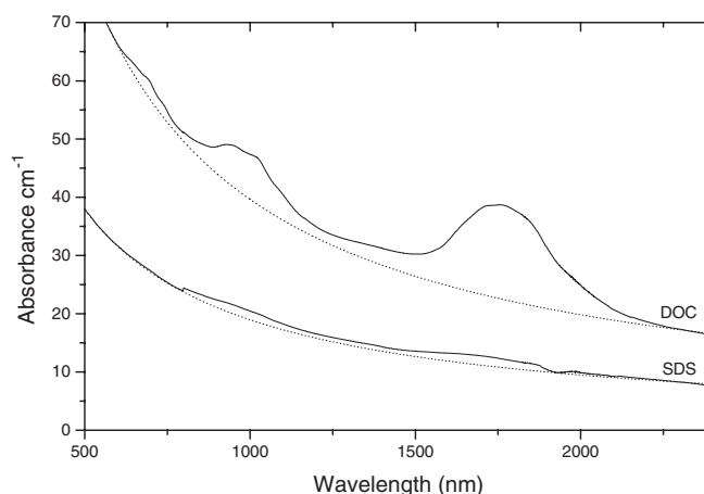
Figure 7. Absorption spectra of two SWNT solutions (using 10 \text{ g L}^{-1} raw SWNT material) in \text{D}_2\text{O} with SDS and with DOC before ultracentrifugation. The 1/\lambda background to be subtracted is also shown (dotted lines) for each spectrum. The dip near 1900 nm is an artifact due to imperfect correction for the solvent absorption.
