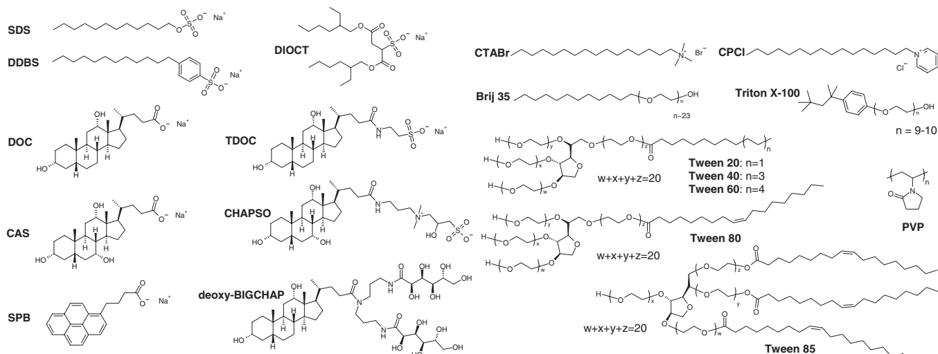
Figure 1. Chemical structures of the surfactants used in this study. Abbreviations: SDS: sodium dodecylsulfate, DDBS: sodium dodecylbenzenesulfonate, DIOCT: dioctyl sulfosuccinate, sodium salt, SPB: sodium pyrenebutyrate, CAS: sodium cholate, DOC: sodium deoxycholate, TDOC: sodium taurodeoxycholate, CTABr: cetyltrimethylammonium bromide, CPCl: cetylpyridinium chloride, PVP: polyvinylpyrrolidone.
