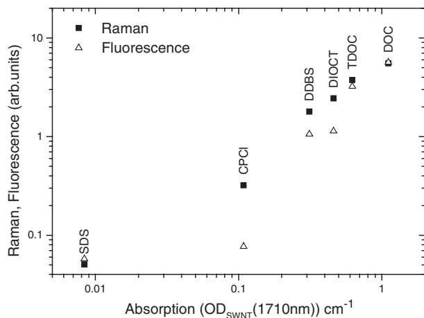
Figure 6. Correlation of integrated fluorescence and Raman intensities with absorbance for the ultracentrifuged SWNT solutions of Figures 3–5.
